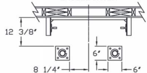
BUFFER SPRING LOCATION EXCELEVATOR
