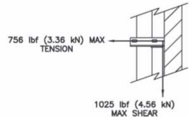
SIDE VIEW OF RAIL BRACKET
